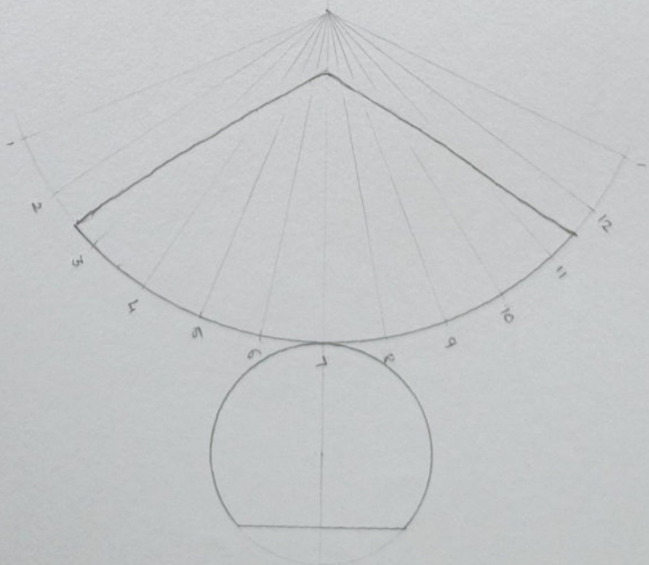
SURFACE DEVELOPMENT
