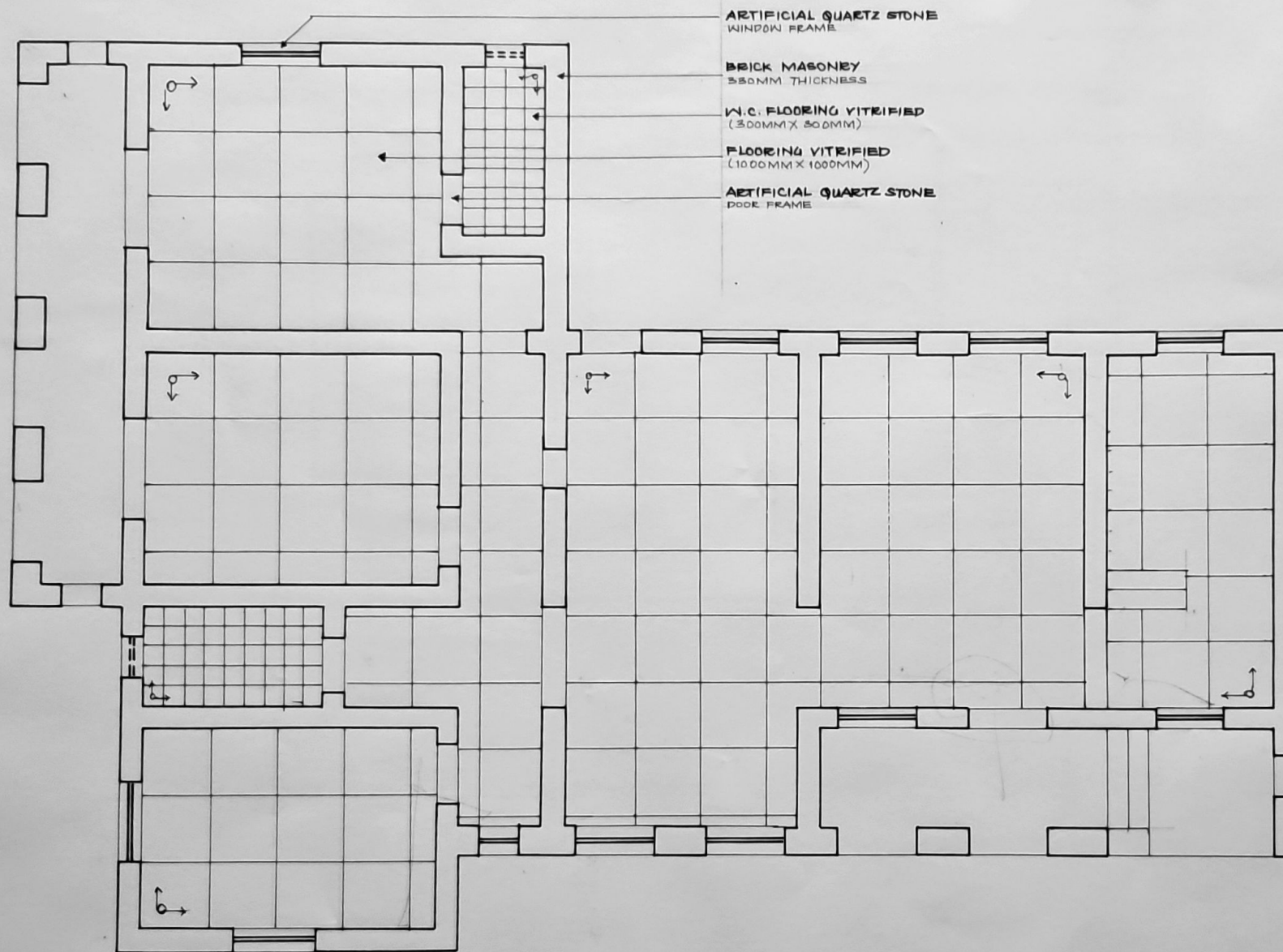
PLAN SCALE - 1:50
