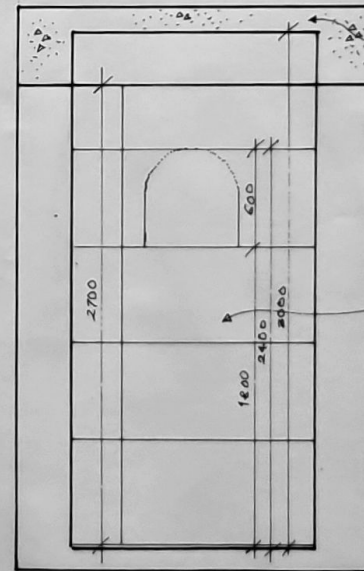
SECTION DD'
