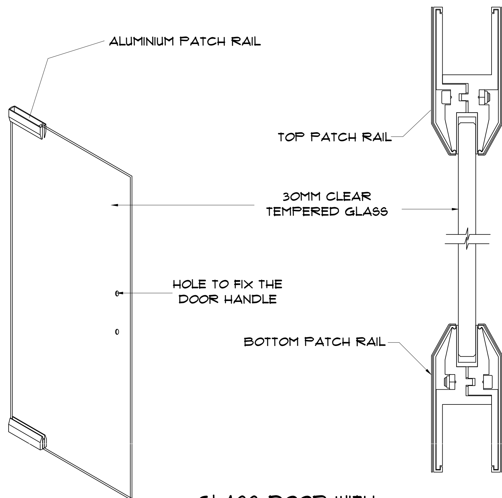
GLASS DOOR WITH ALUMINIUM PATCH RAIL SCALE - 1:4
