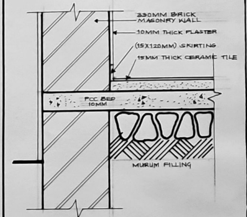
FLOORING DETAIL
