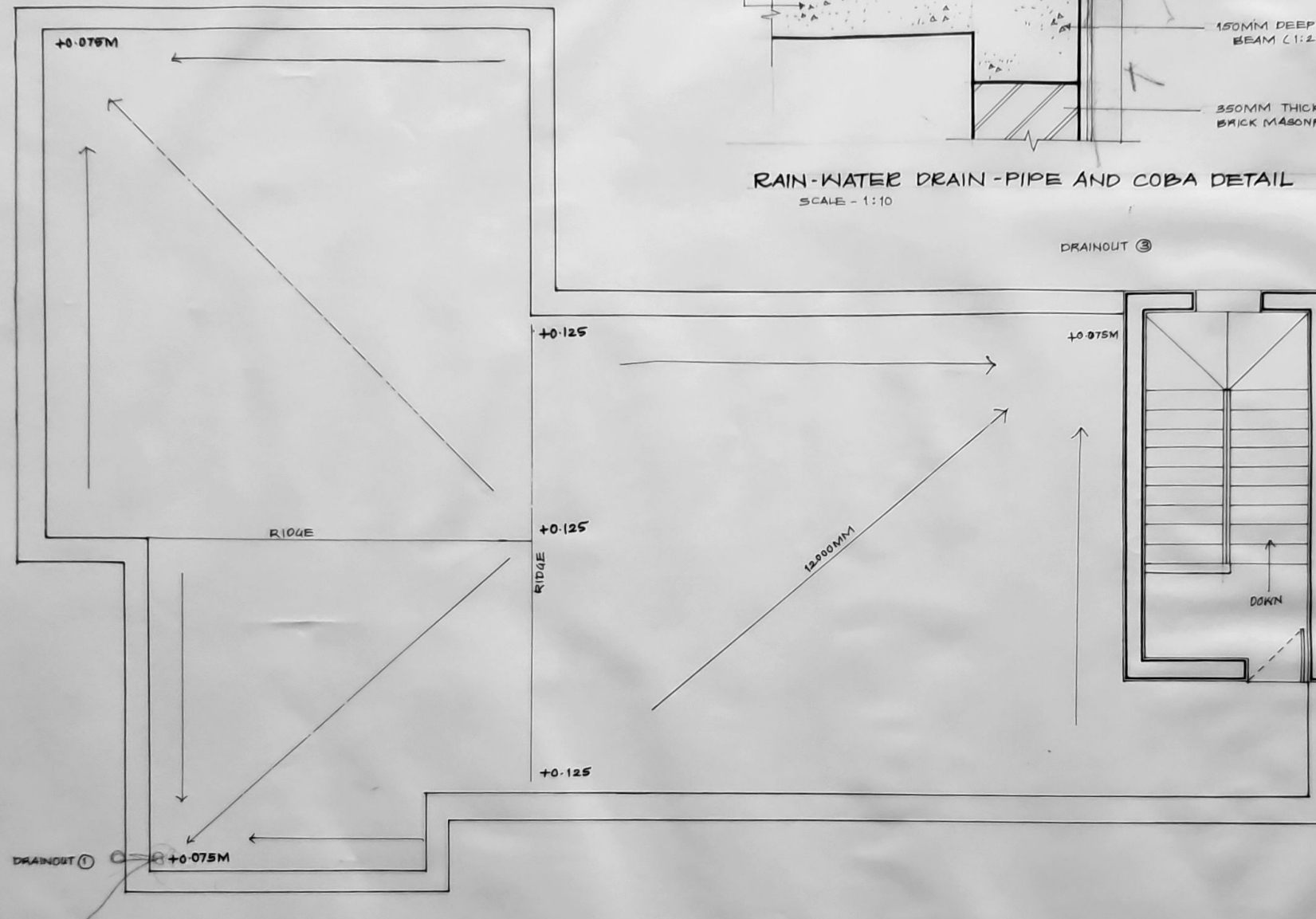
TERRACE PLAN
