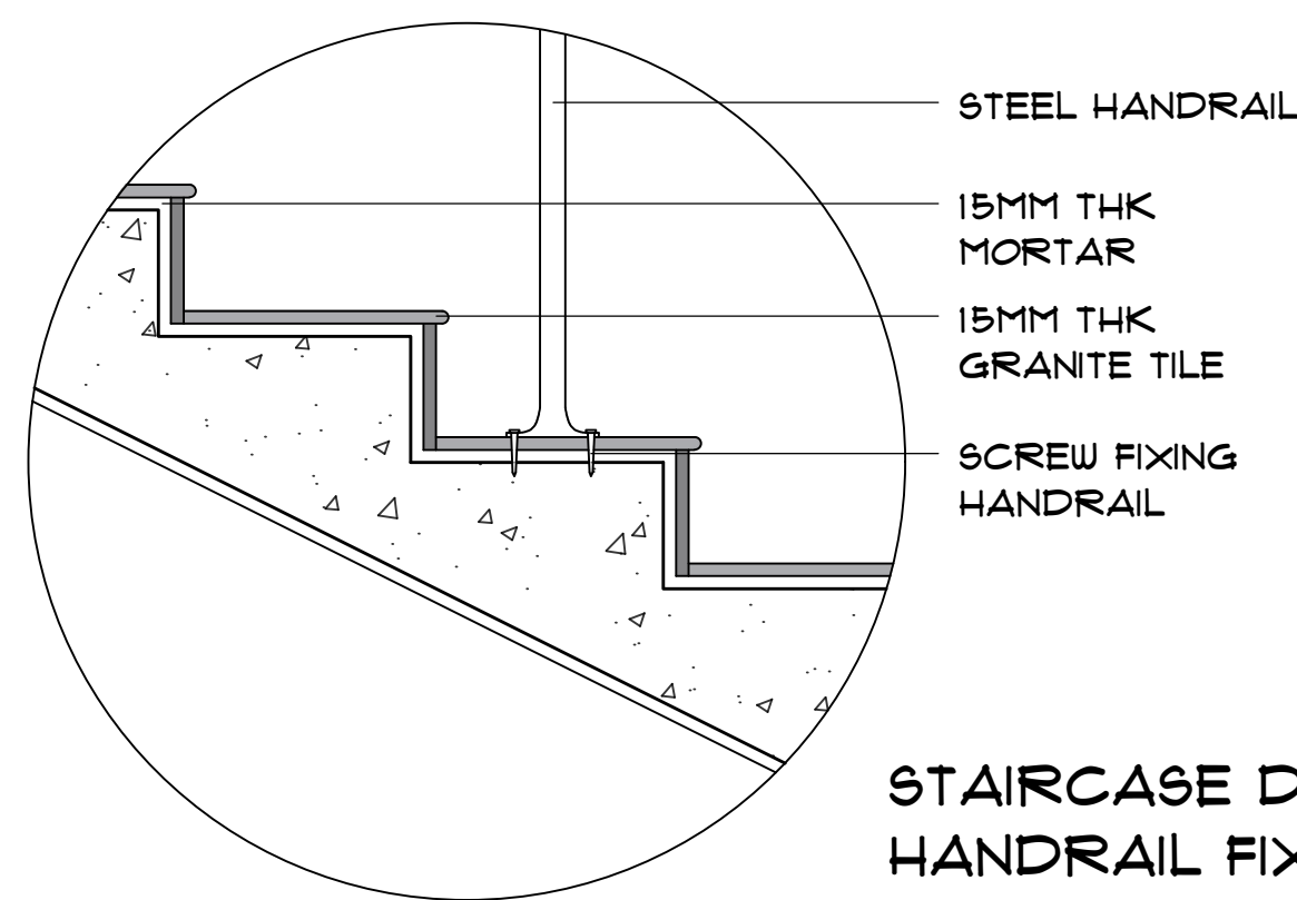
STAIRCASE SECTION EE' SCALE - 1:30
