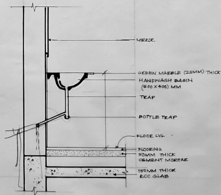
WASH-BASIN DETAIL
